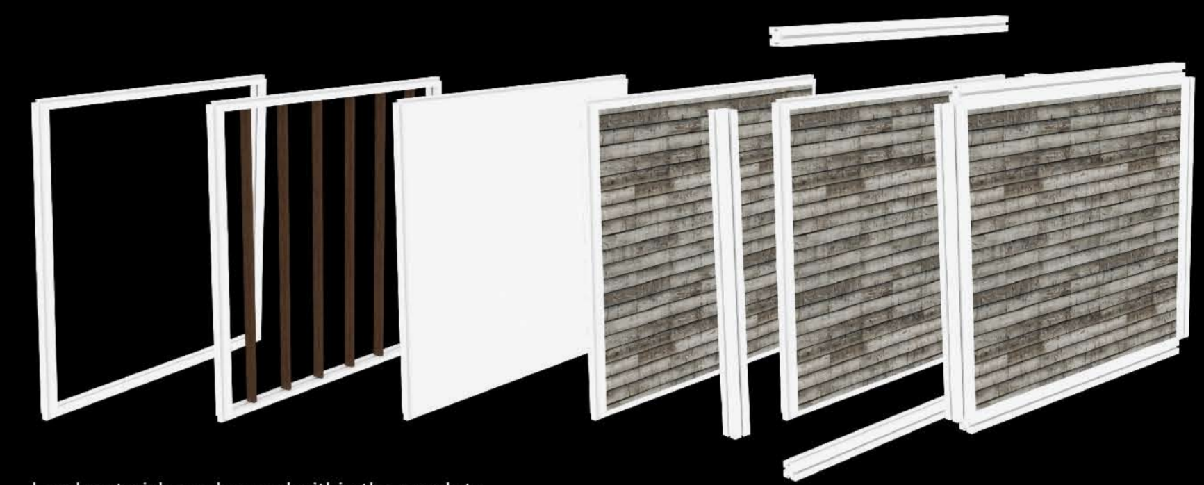
Local materials can be used within the panels to celebrate sustainable Canadian construction techniques and culturally significant building practices
